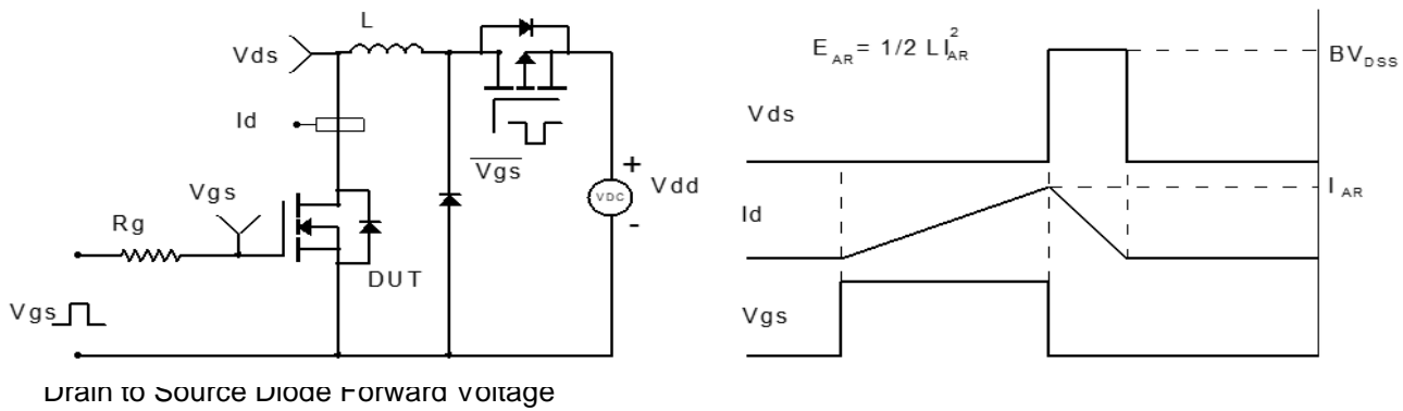
Figure 3: Unclamped Inductive Switching Test Circuit & Waveform
