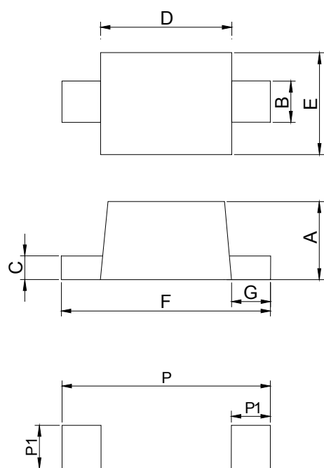
Land Pattern
