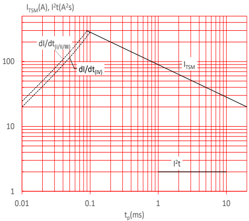
FIG.6: Non-repetitive surge peak on-state current for a sinusoidal pulse with width t_p < 20\text{ms} , and corresponding value of I^2t ( I - II -III: dl/dt < 50\text{A}/\mu\text{s} ; IV: dl/dt < 30\text{A}/\mu\text{s} )
