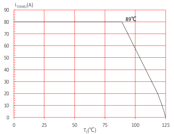
FIG.4: On-state characteristic
