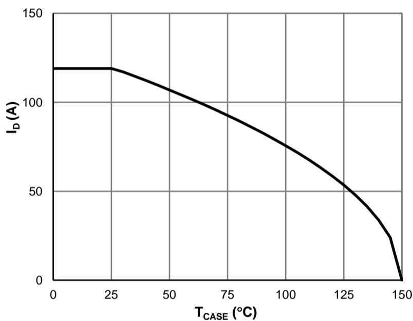
Figure 9: Current De-rating
