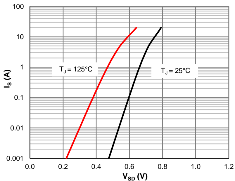
Figure 7: Body-Diode Characteristics
