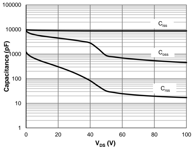
Figure 8: Capacitance Characteristics
