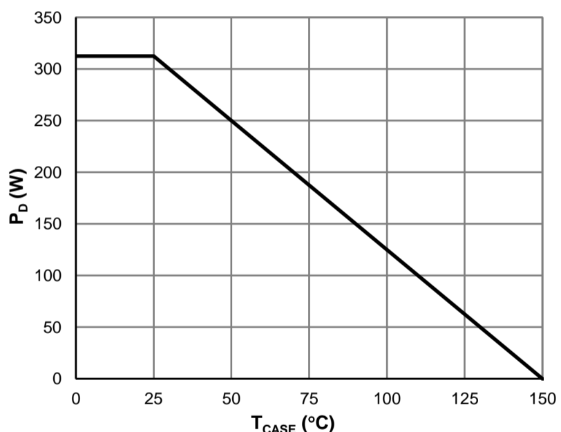
Figure 10: Power De-rating
