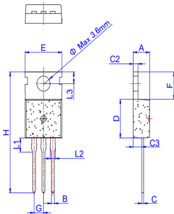
TO-220C
