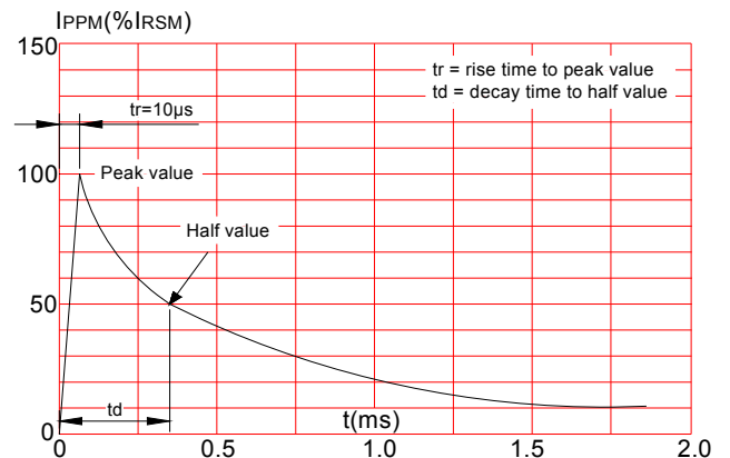
FIG.4: Pulse waveform
