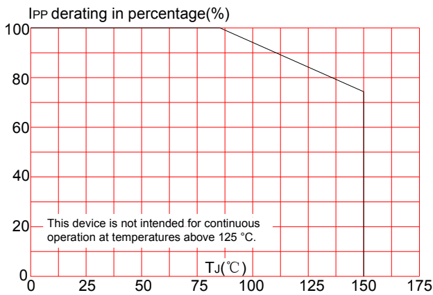
FIG.5: Pulse derating curve(8/20μs)
