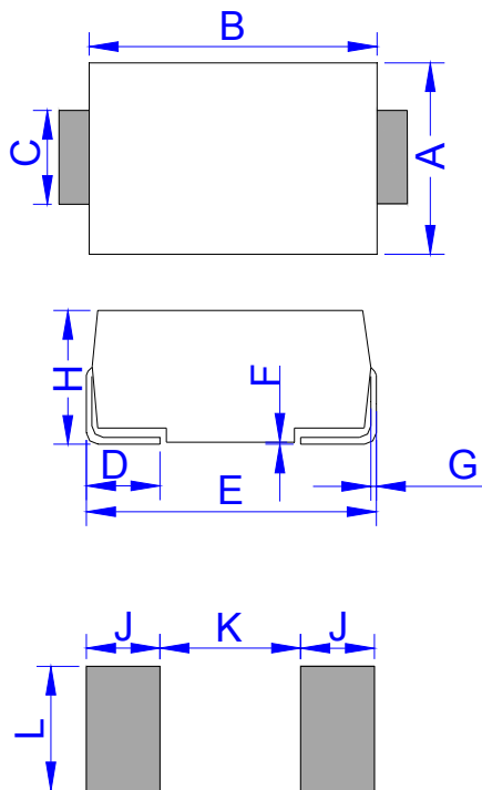
DO-214AA (SMB)
