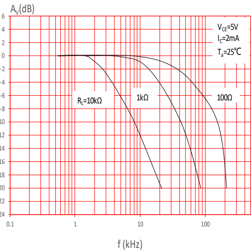
FIG.10: Frequency Response
