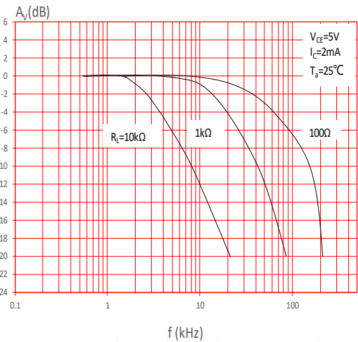
FIG.10: Frequency Response
