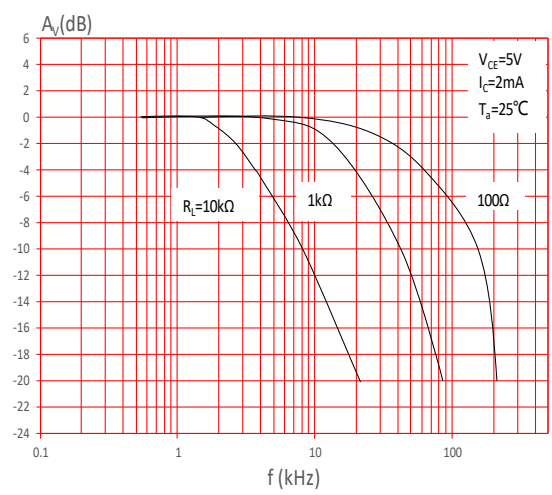
FIG.10: Frequency Response
