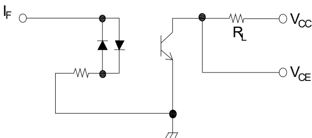
FIG.11: Test Circuits of Response Time
