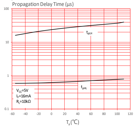
FIG.12: Propagation Delay Time vs. Ambient Temperature
