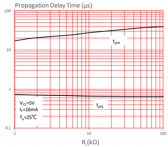
FIG.10: Propagation Delay Time vs. Load Resistance
