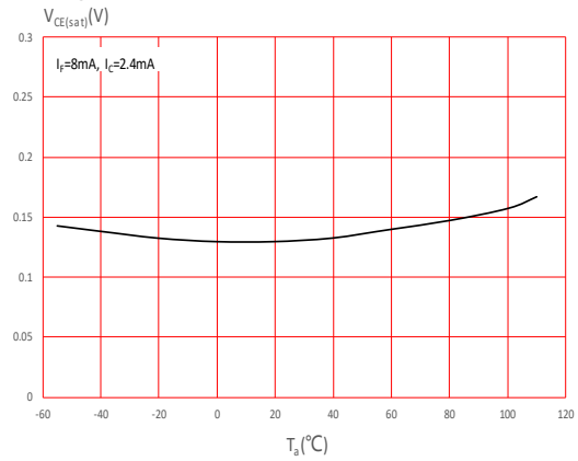
FIG.8: Normalized Collector-emitter Saturation Voltage vs. Ambient Temperature
