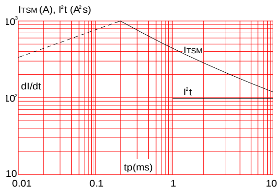
FIG.5: Non-repetitive surge peak on-state current for a sinusoidal pulse with width t_p < 10\text{ms} , and corresponding value of f t ( di/dt < 100\text{A}/\mu\text{s} )
