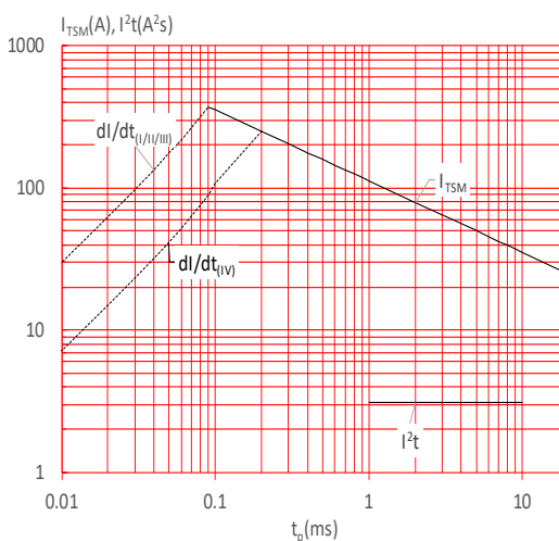
FIG.6: Non-repetitive surge peak on-state current for a sinusoidal pulse with width t_p < 20\text{ms} , and corresponding value of I^2t (I - II - III: di/dt < 80\text{A}/\mu\text{s} ; IV: di/dt < 40\text{A}/\mu\text{s} )
