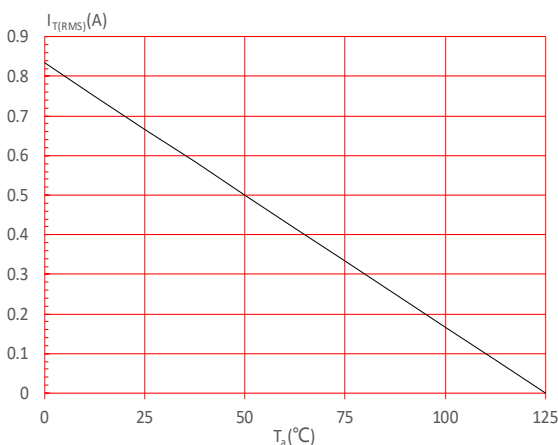
FIG.5: On-state characteristics
