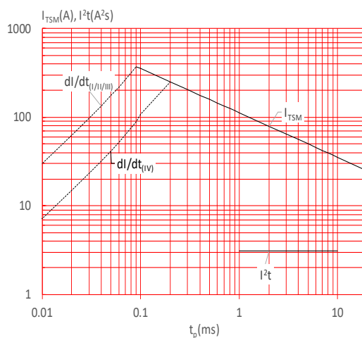
FIG.6: Non-repetitive surge peak on-state current for a sinusoidal pulse with width t_p < 20ms , and corresponding value of I^2t (I - II - III: dI/dt < 50A/\mu s ; IV: dI/dt < 40A/\mu s )
