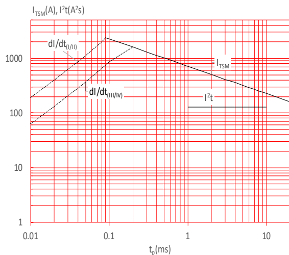
FIG.5: Non-repetitive surge peak on-state current for a sinusoidal pulse with width t_p < 20\text{ms} , and corresponding value of I^2t (I - II : di/dt < 80\text{A}/\mu\text{s} ; III-IV : di/dt < 40\text{A}/\mu\text{s} )
