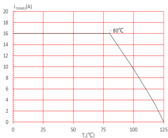
FIG.4: On-state characteristics
