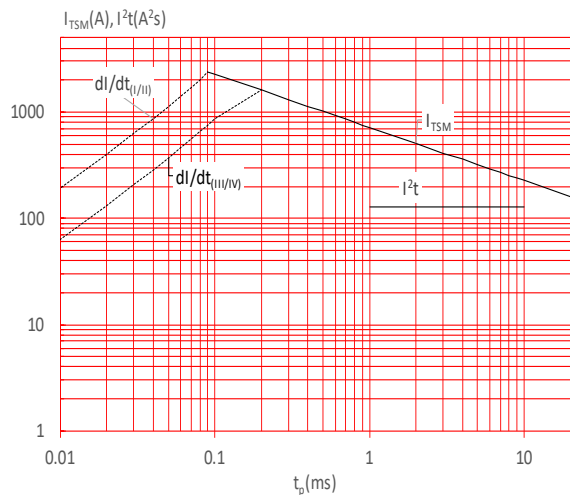
FIG.5: Non-repetitive surge peak on-state current for a sinusoidal pulse with width t_p < 20\text{ms} , and corresponding value of I^2t (I - II: di/dt < 80\text{A}/\mu\text{s} ; III-IV: di/dt < 40\text{A}/\mu\text{s} )
