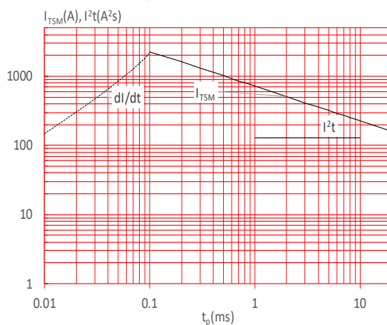
FIG.6: Non-repetitive surge peak on-state current for a sinusoidal pulse with width t_p < 20\text{ms} , and corresponding value of I^2t ( dl/dt < 50\text{A}/\mu\text{s} )
