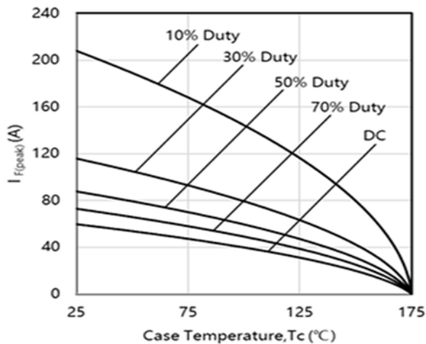
FIG.8: Current derating
