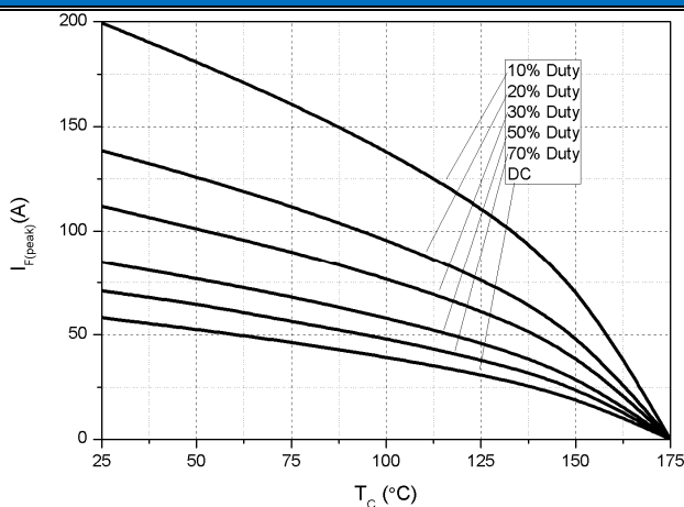
FIG.8: Current derating
