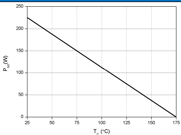
FIG.7: Power derating
