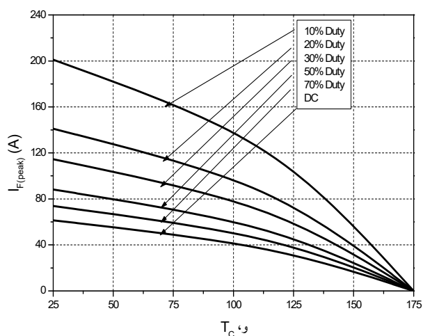
FIG.7: Current derating
