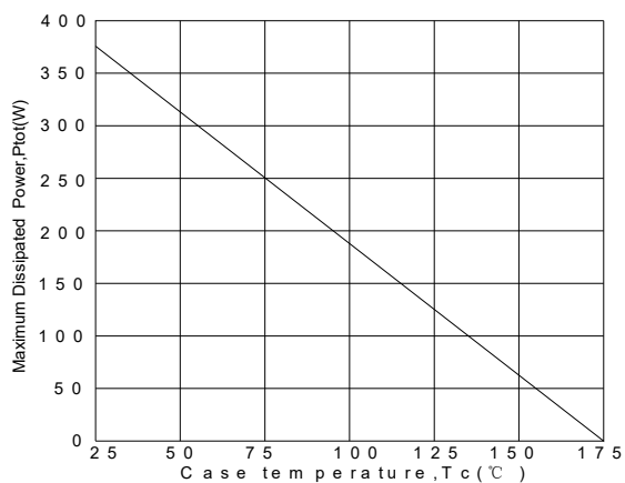
FIG.7: Power derating
