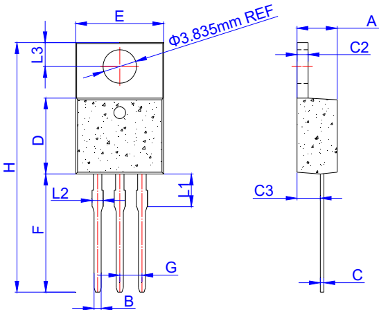
TO-220AB
