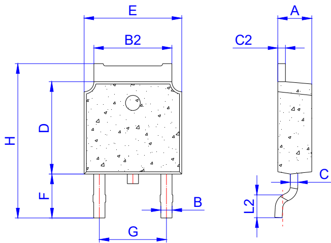
TO-252
