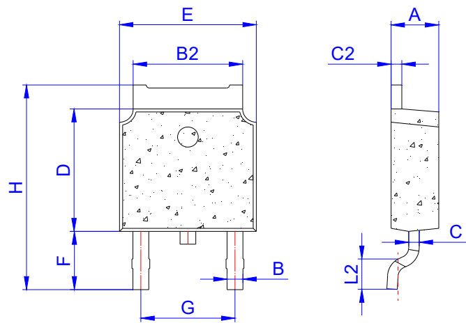
TO-252
