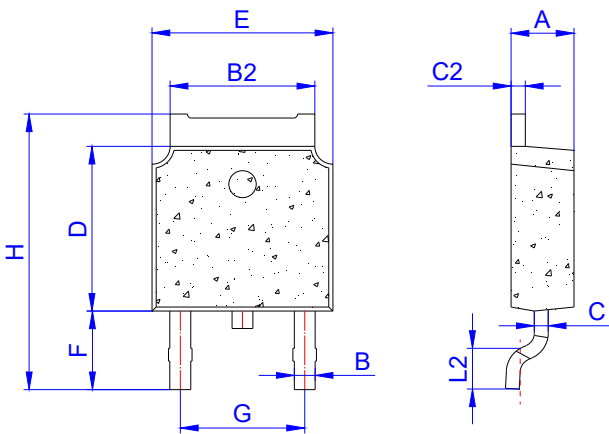
TO-252
