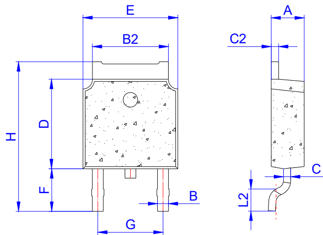
TO-252
